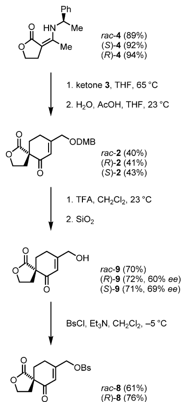
Scheme 3. Robinson annulation, deprotection, and determination of absolute configuration. DMB = 3,4-(MeO) 2 C 6 H 3 CH 2 –, Bs = 4-BrC 6 H 4 SO 2 –.
