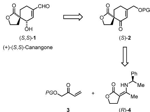
Scheme 1. Synthetic plan for optically active (+)-( S,S )-canangone ( 1 ) by an asymmetric Robinson annulation reaction with the use of ( R )-phenethylamine as a chiral auxiliary. PG = protecting group.
