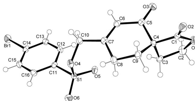
Figure 1. ORTEP view of optically active brosylate 8 . The depicted enantiomer has the ( R ) configuration.
