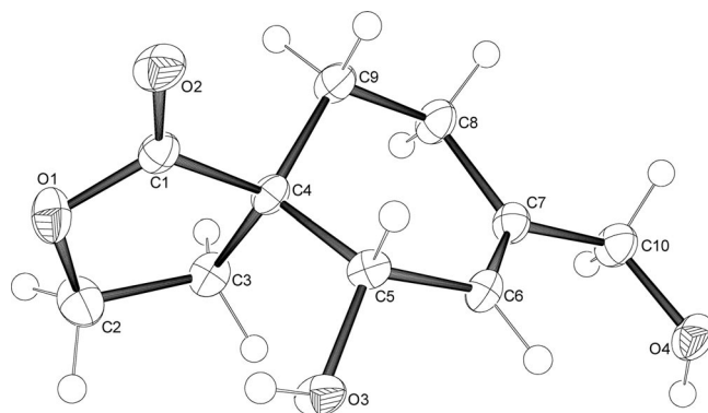
Figure 2. ORTEP view of racemic diol ( R *, S *)- 10 . The depicted enantiomer has the ( 5R,6S ) configuration.
