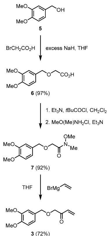
Scheme 2. Synthesis of protected Michael acceptor 3 .
